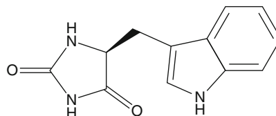
L-5-Indolylmethylhydantoin
