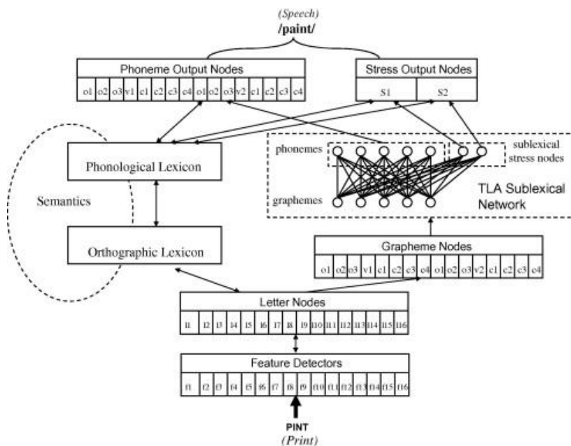
Figure 2. The CDP++ model (Perry, Ziegler, and Zorzi, 2010).
