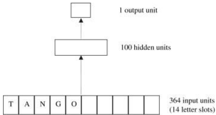
Figure 3. The Ševa et al. (2009) network of stress assignment.
