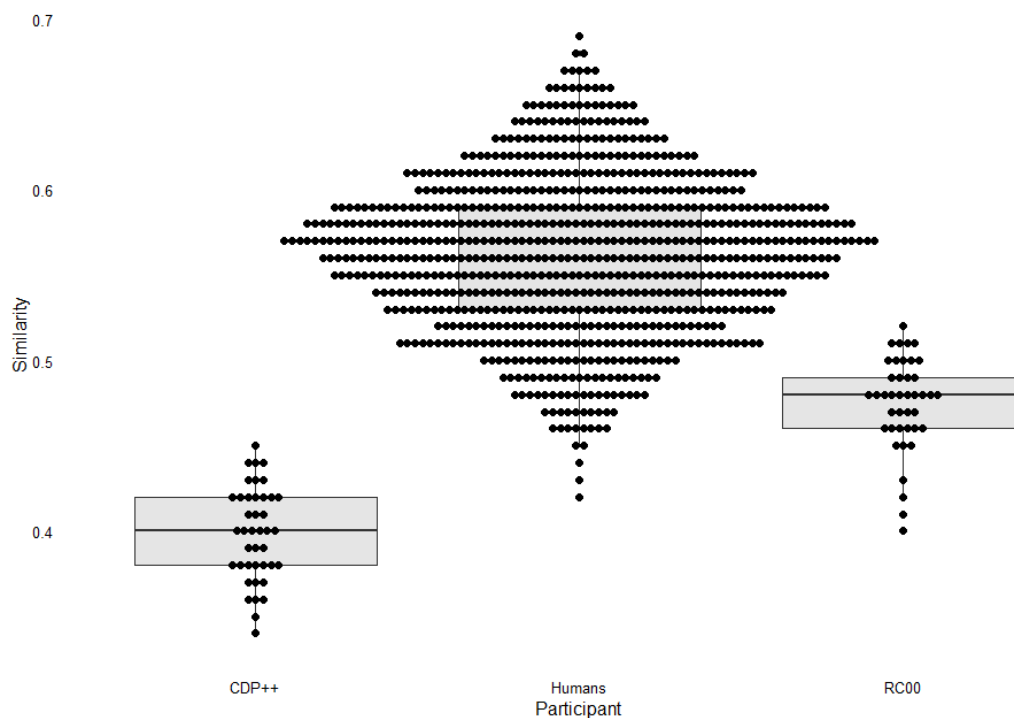
Figure 5. Pronunciation similarity between participants and between models and every other participant.
