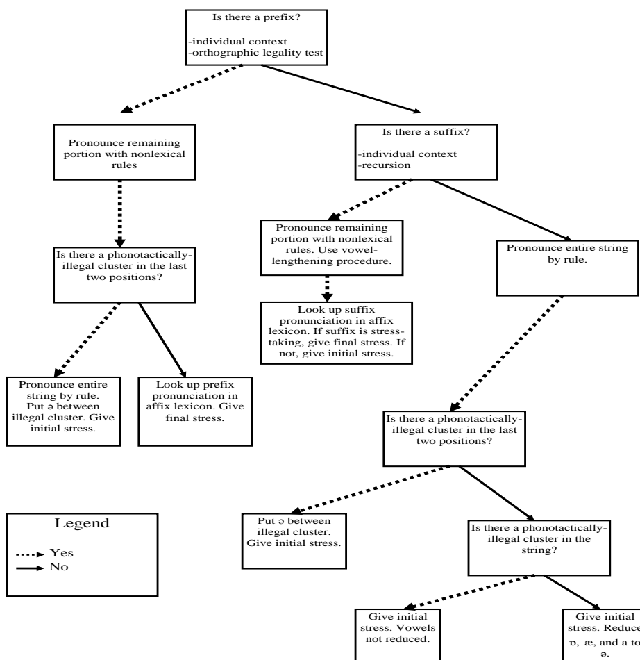
Figure 1. The rule-based algorithm of Rastle and Coltheart (2000).
