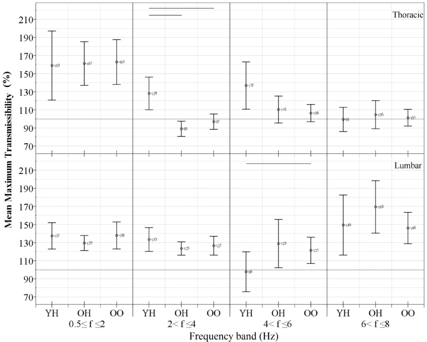
Figure 1 Mean maximum transmissibility of the lumbar and thoracic spines at frequency bands. — = significant difference between groups. Dotted line= 100% transmissibility, attenuation below and amplification above. Young and healthy (YH), older healthy (OH), older osteoporotic (OO). 95% error bars and mean presented.
