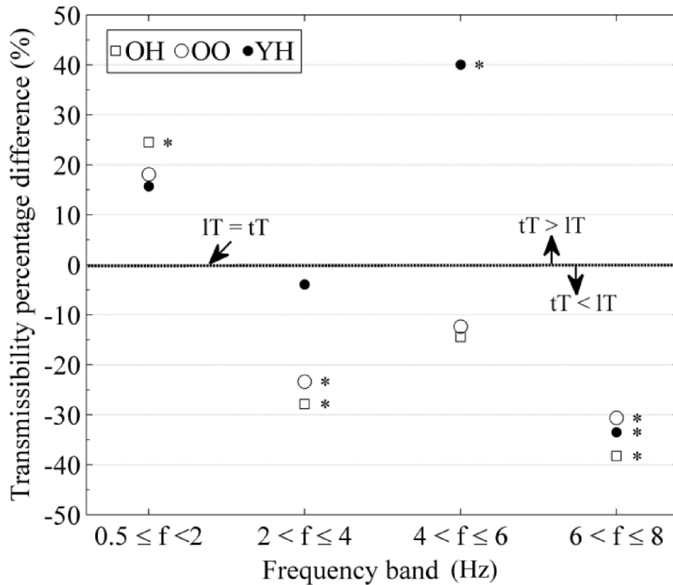
Figure 3 Percentage differences in mean maximum transmissibility (T) between thoracic (t) and lumbar spines (l) at various frequency bands. *=significant difference in T between l and t. Young and healthy (YH), older healthy (OH), older osteoporotic (OO)
